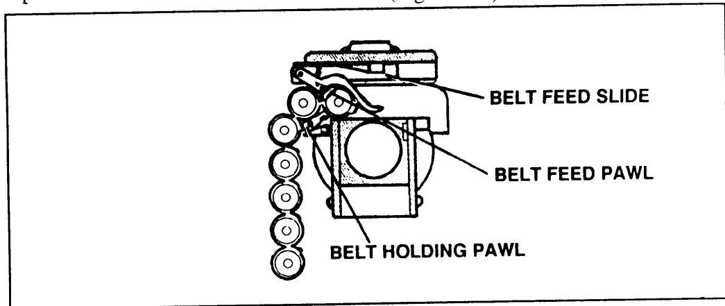
Figure 3-6. Feeding—step 2.
